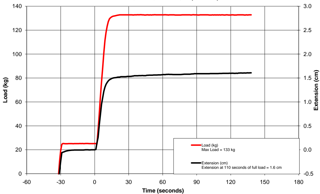
Low Temperature Retention Testing 10/07/11 JIAN212, ZOX, FF392, L ( 52 cm)
