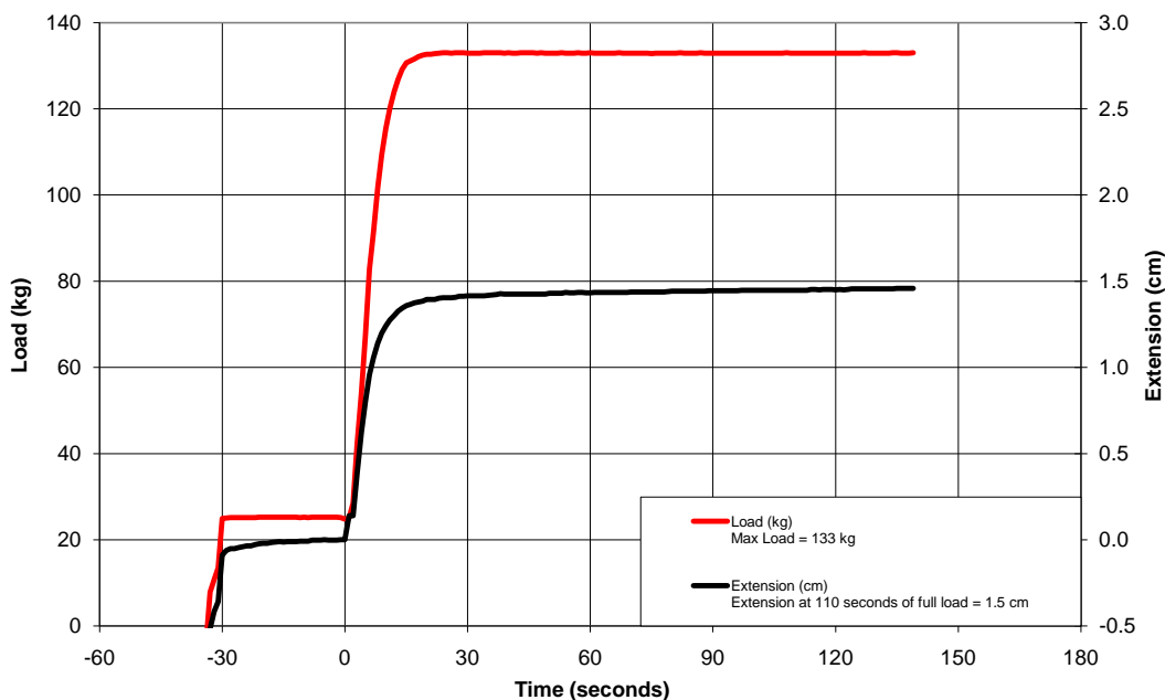
Ambient Temperature Retention Testing 10/07/11 JIAN212, ZOX, FF392, L ( 52 cm)
