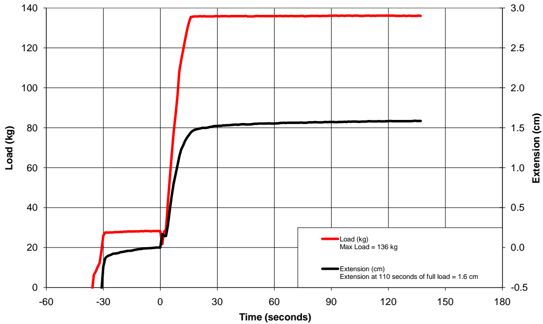
Ambient Temperature Retention Testing 02/15/11 JIAN167, MHR, LS2 OF569, M (58 cm)
