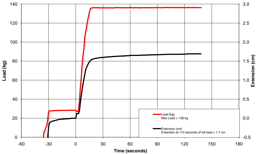
Low Temperature Retention Testing 02/15/11 JIAN167, MHR, LS2 OF569, M (58 cm)
