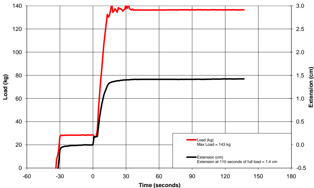
Ambient Temperature Retention Testing 01/27/11 JIAN158, MHR, LS2 FF385, XXXXL (66 cm)
