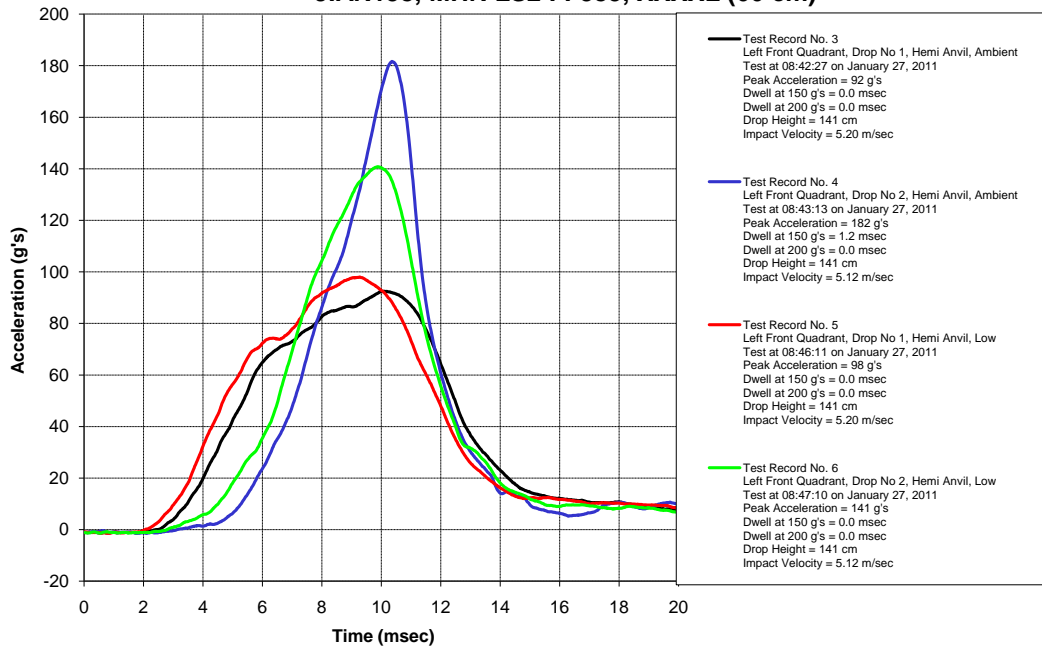
Impact Testing JIAN158, MHR LS2 FF385, XXXXL (66 cm)
