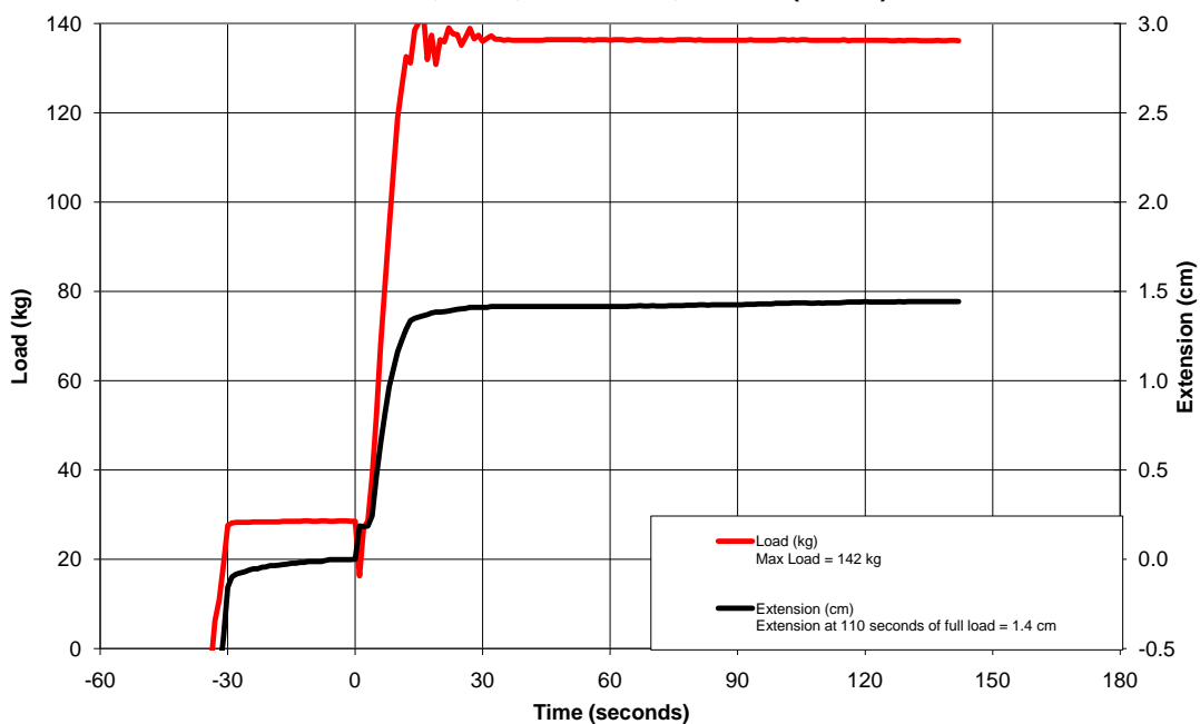
Low Temperature Retention Testing 01/27/11 JIAN158, MHR, LS2 FF385, XXXXL (66 cm)
