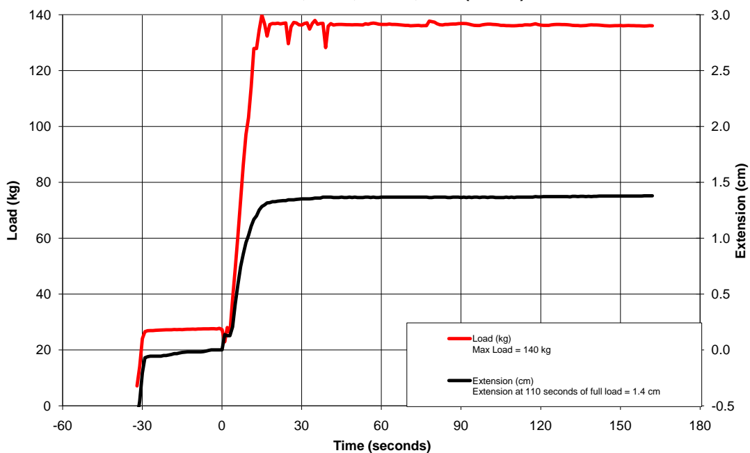
Low Temperature Retention Testing 09/02/10 JIAN144, MHR, FF385, XXL (64 cm)
