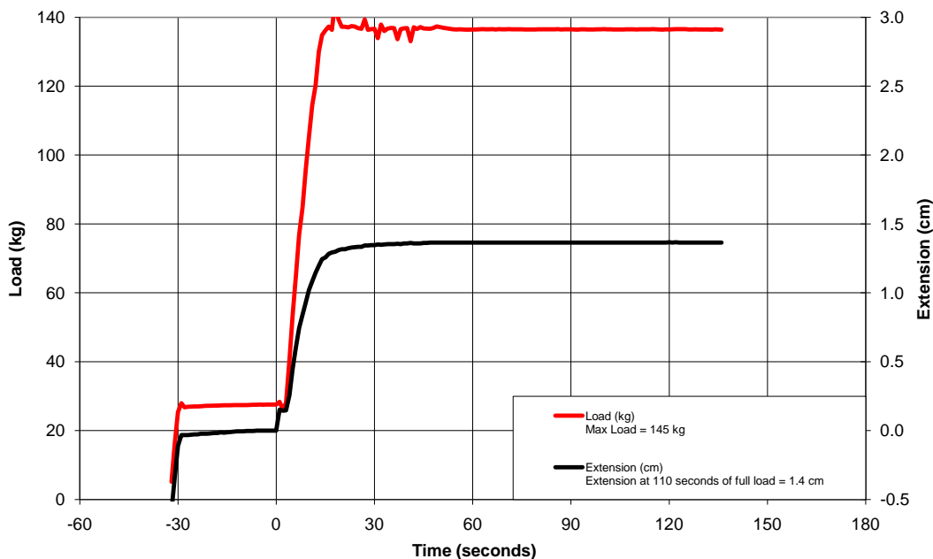
Ambient Temperature Retention Testing 09/02/10 JIAN144, MHR, FF385, XXL (64 cm)
