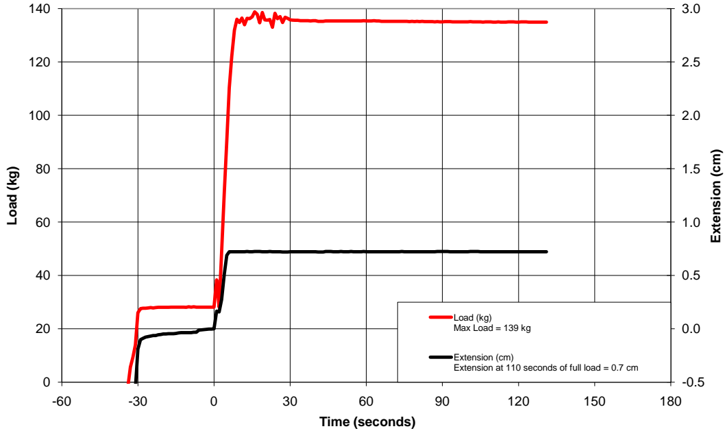
Ambient Temperature Retention Testing 01/25/11 JIAN156, MHR, LS2 FF385, M (58 cm)
