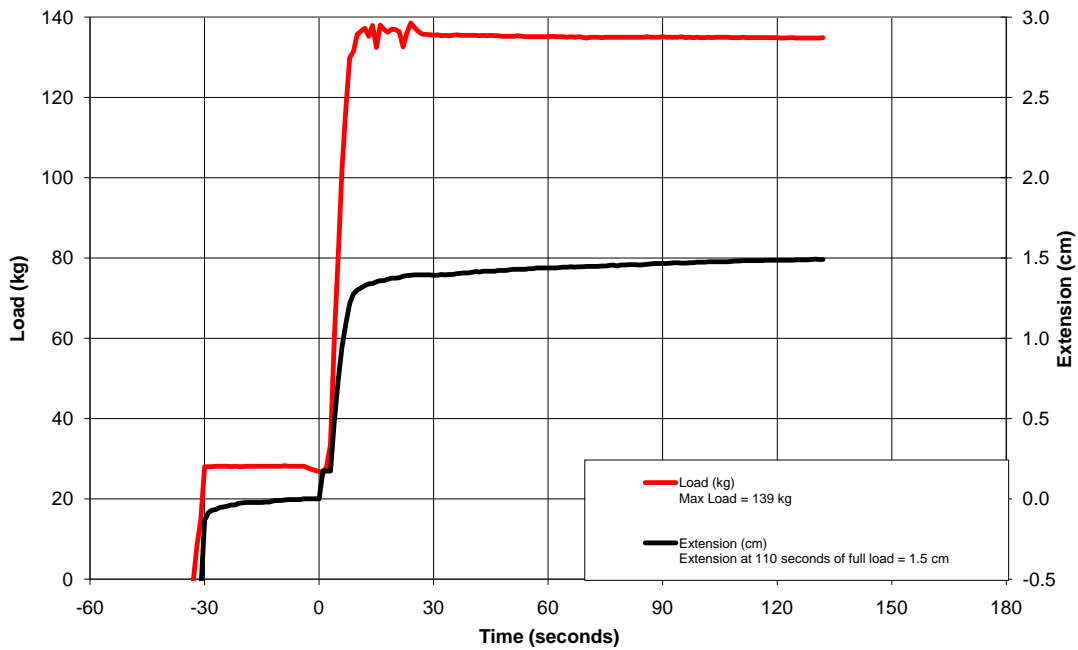
Low Temperature Retention Testing 01/25/11 JIAN156, MHR, LS2 FF385, M (58 cm)
