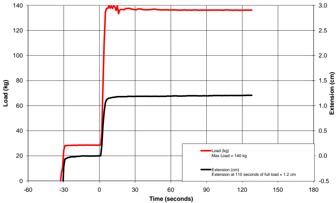
Low Temperature Retention Testing 02/07/11 JIAN161, MHR, LS2 FF386, XXXXL (66cm)
