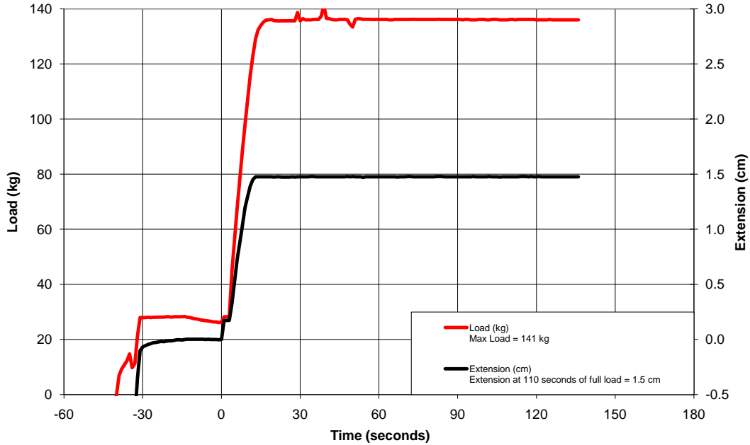
Ambient Temperature Retention Testing 02/07/11 JIAN161, MHR, LS2 FF386, XXXXL (66cm)
