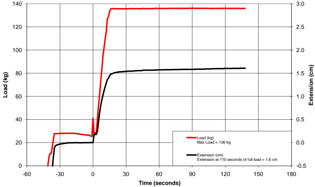
Ambient Temperature Retention Testing 01/31/11 JIAN160, MHR, LS2 FF386, XXL (64cm)
