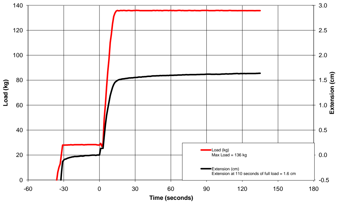
Low Temperature Retention Testing 01/31/11 JIAN160, MHR, LS2 FF386, XXL (64cm)
