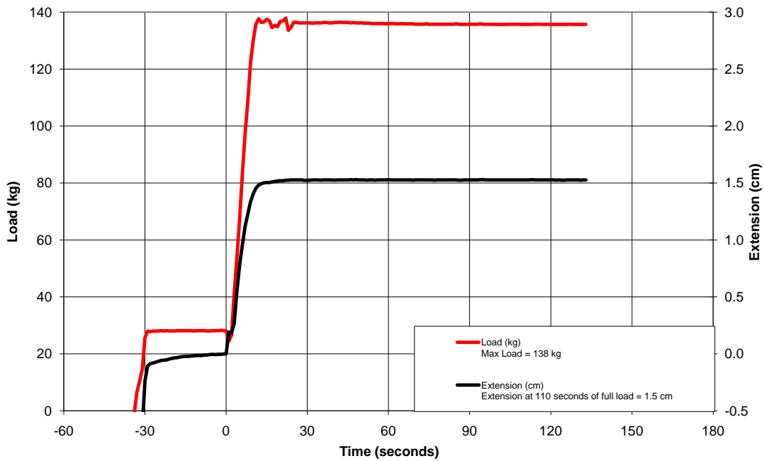
Low Temperature Retention Testing 01/28/11 JIAN159, MHR, LS2 FF386, M (58 cm)
