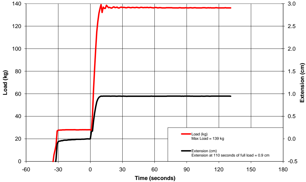
Ambient Temperature Retention Testing 01/28/11 JIAN159, MHR, LS2 FF386, M (58 cm)
