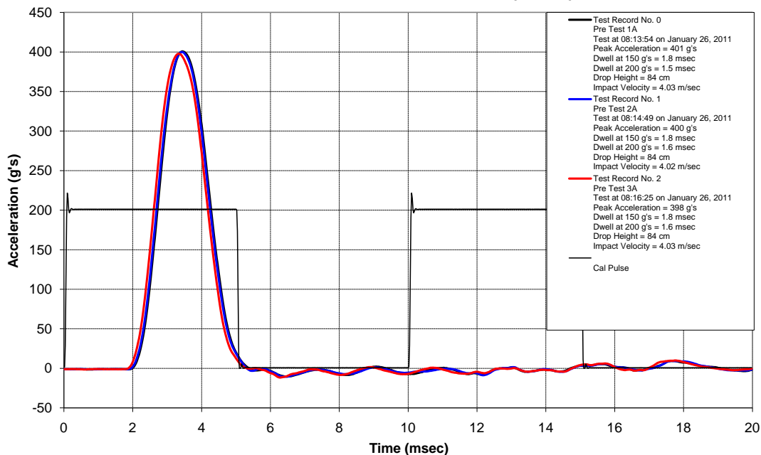
Impact Testing JIAN157, MHR LS2 FF385, XXL (64 cm)
