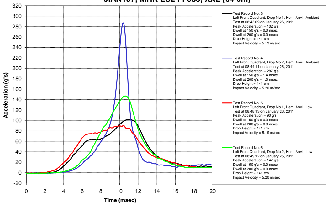
Impact Testing JIAN157, MHR LS2 FF385, XXL (64 cm)
