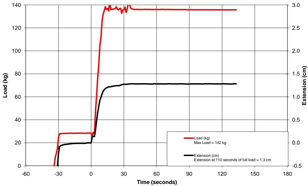
Low Temperature Retention Testing 01/26/11 JIAN157, MHR, LS2 FF385, XXL (64 cm)
