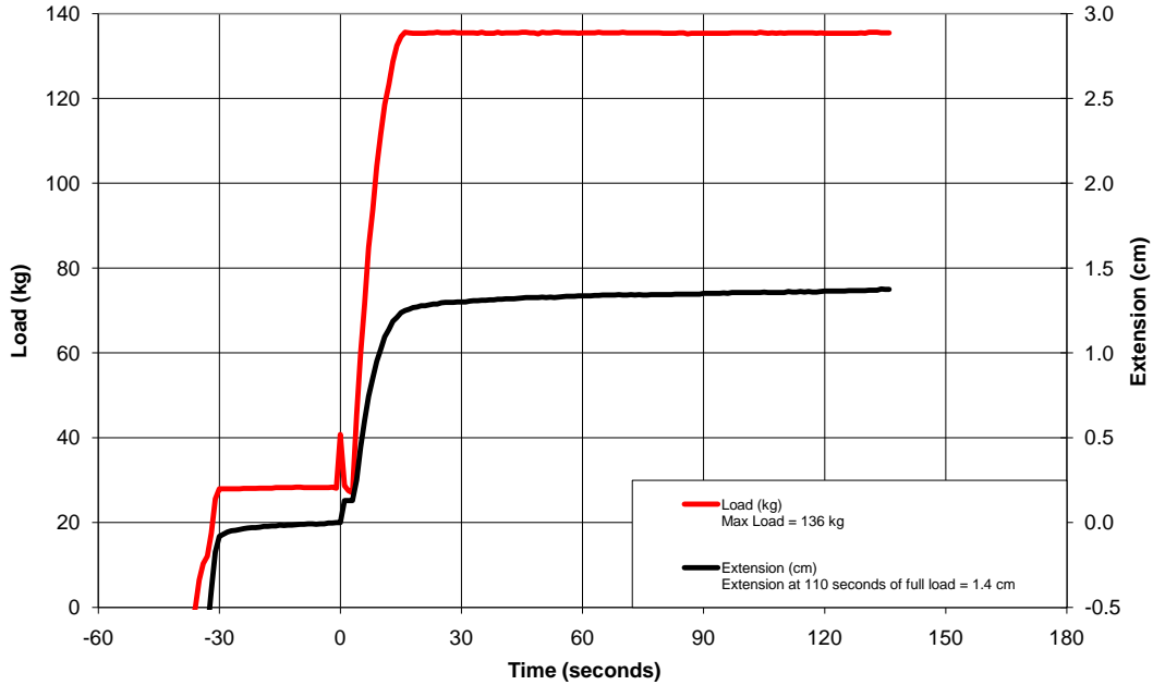
Ambient Temperature Retention Testing 01/26/11 JIAN157, MHR, LS2 FF385, XXL (64 cm)
