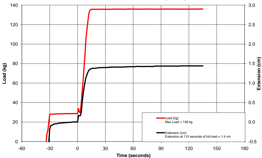
Low Temperature Retention Testing 03/15/11 JIAN173, MHR, LS2 FF385, M (58 cm)
