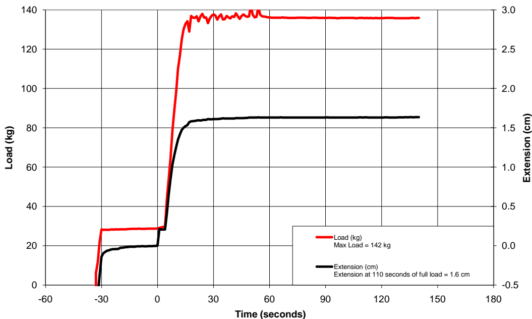
Ambient Temperature Retention Testing 03/15/11 JIAN173, MHR, LS2 FF385, M (58 cm)
