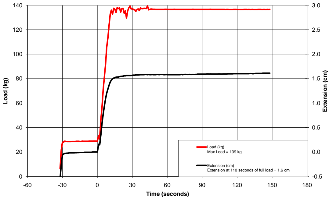
Low Temperature Retention Testing 03/10/11 JIAN170, MHR, LS2 FF385, XXL (64 cm)
