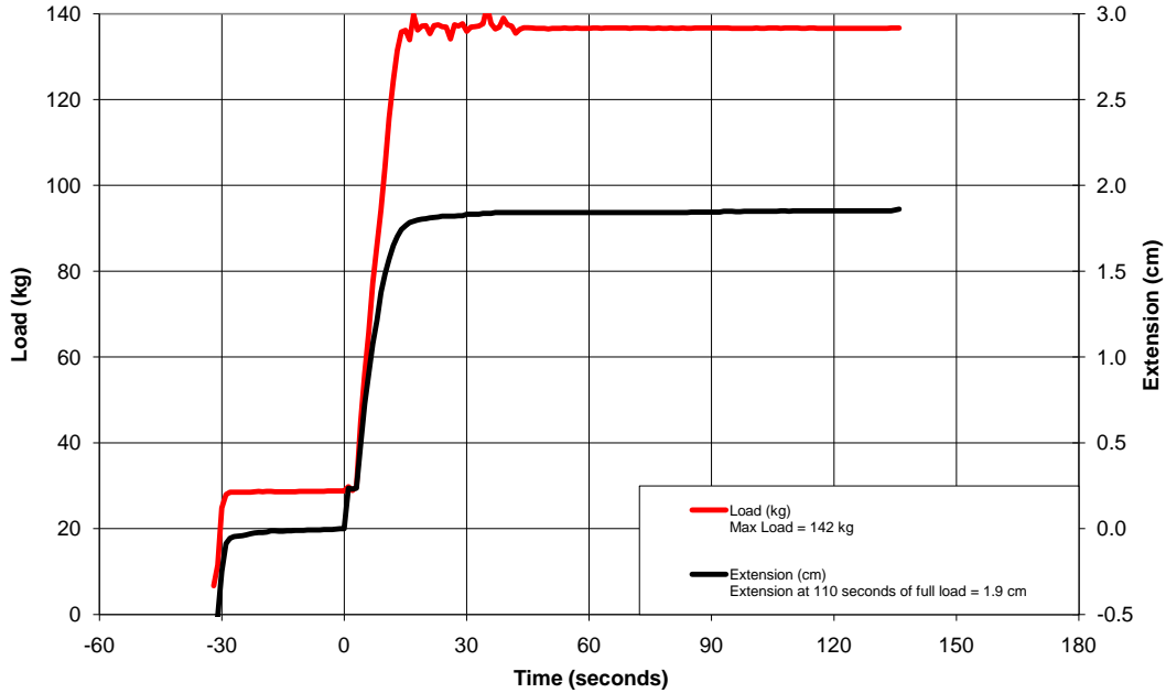
Ambient Temperature Retention Testing 03/10/11 JIAN170, MHR, LS2 FF385, XXL (64 cm)
