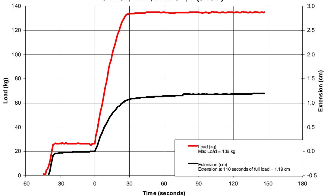
Low Temperature Retention Testing 06/11/08 JIAN31, MHR, MX426-1, L (52 cm)
