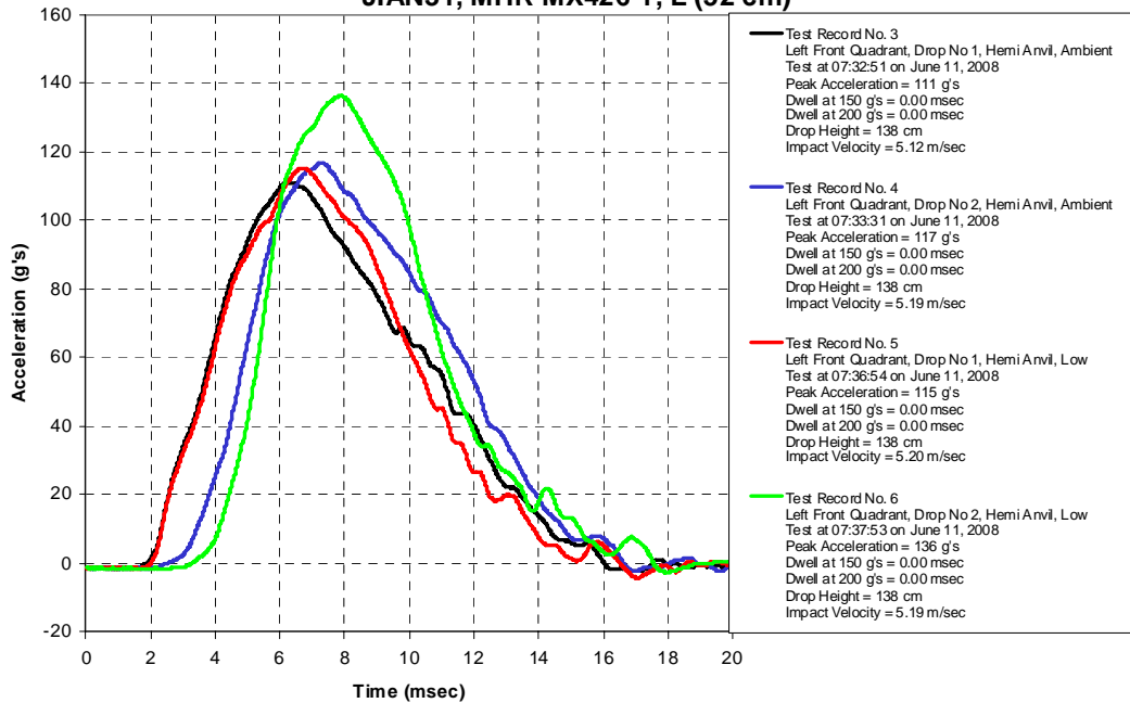
Impact Testing JIAN31, MHR MX426-1, L (52 cm)
