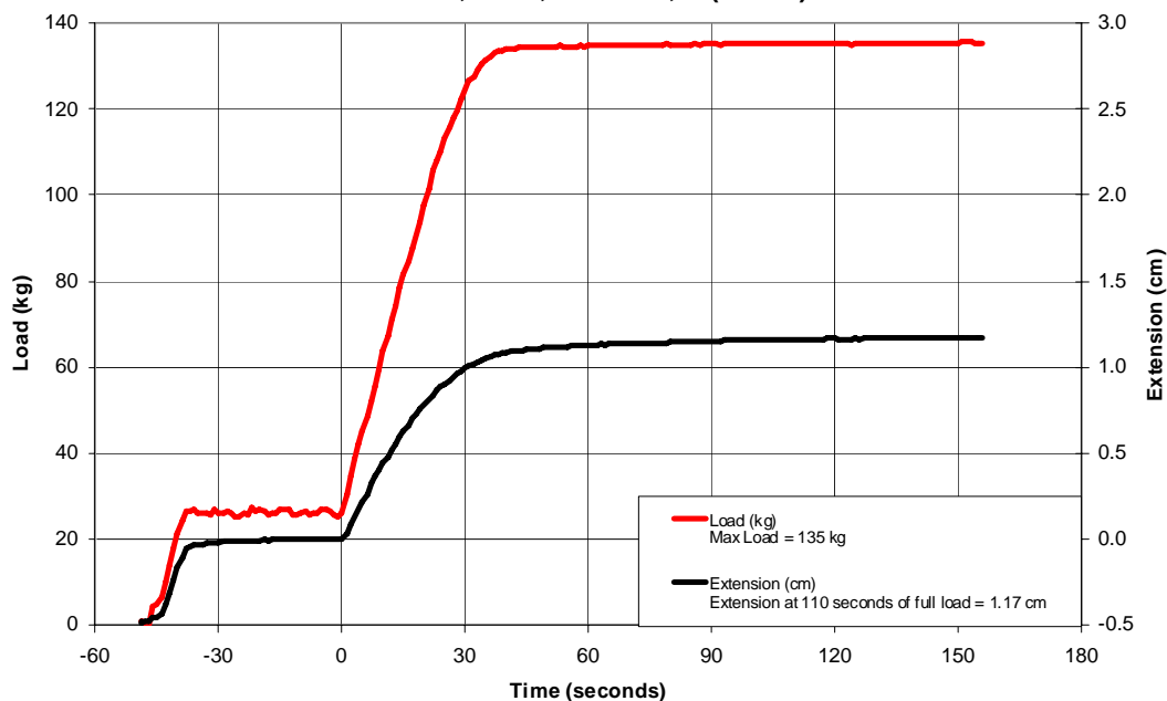
Ambient Temperature Retention Testing 06/11/08 JIAN31, MHR, MX426-1, L (52 cm)
