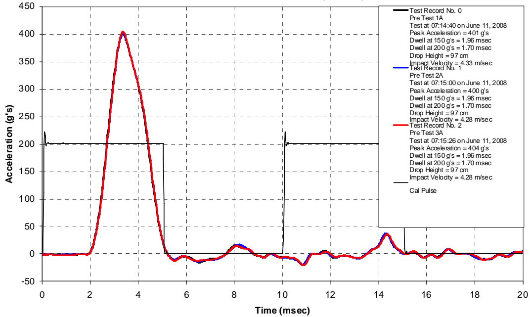
Impact Testing JIAN31, MHR MX426-1, L (52 cm)
