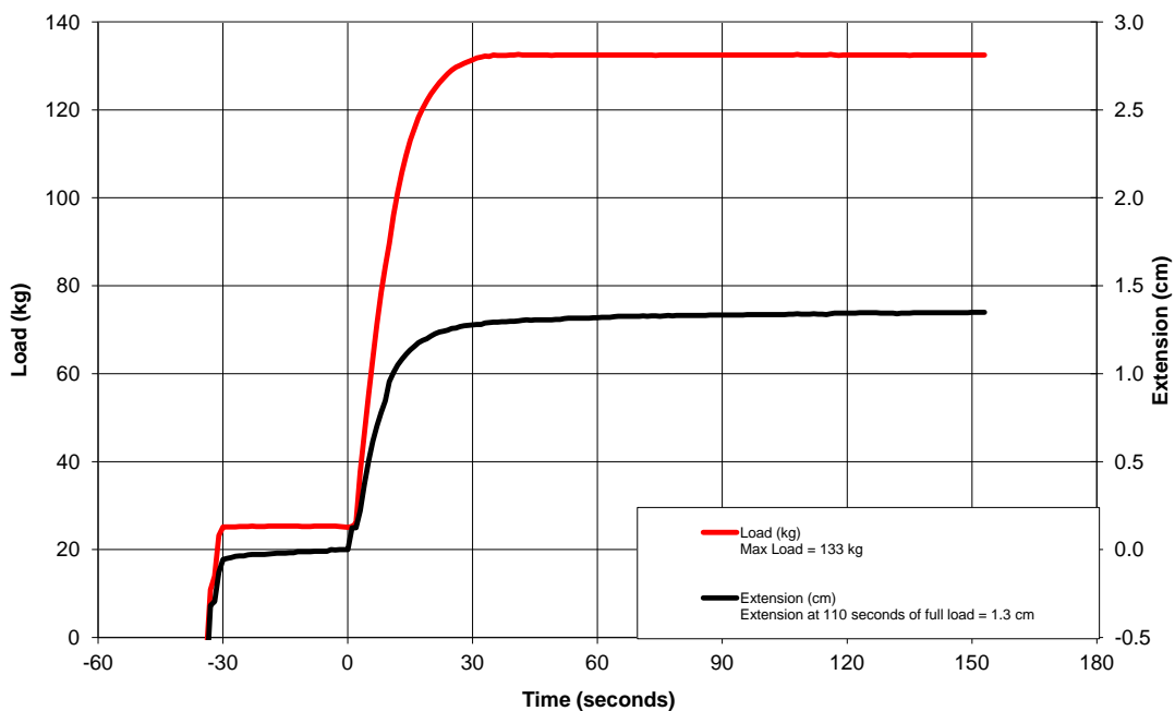
Low Temperature Retention Testing 01/06/12 JIAN214, LS2, FF387, XXXXXL
