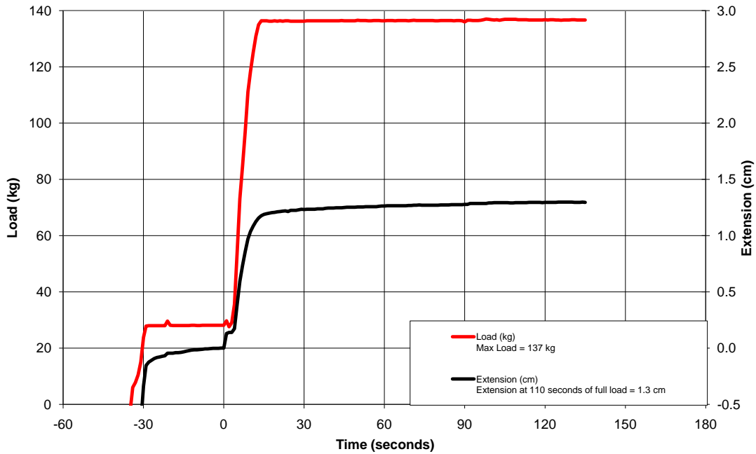
Low Temperature Retention Testing 07/11/11 JIAN201, LS2, OF566, S (56cm)
