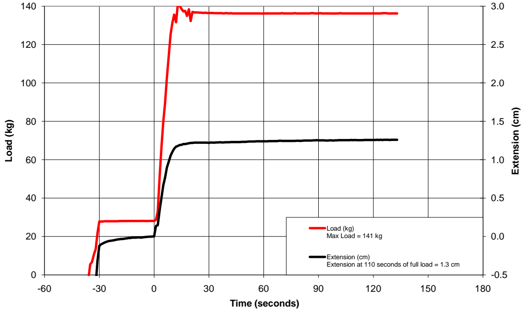
Ambient Temperature Retention Testing 07/11/11 JIAN201, LS2, OF566, S (56cm)
