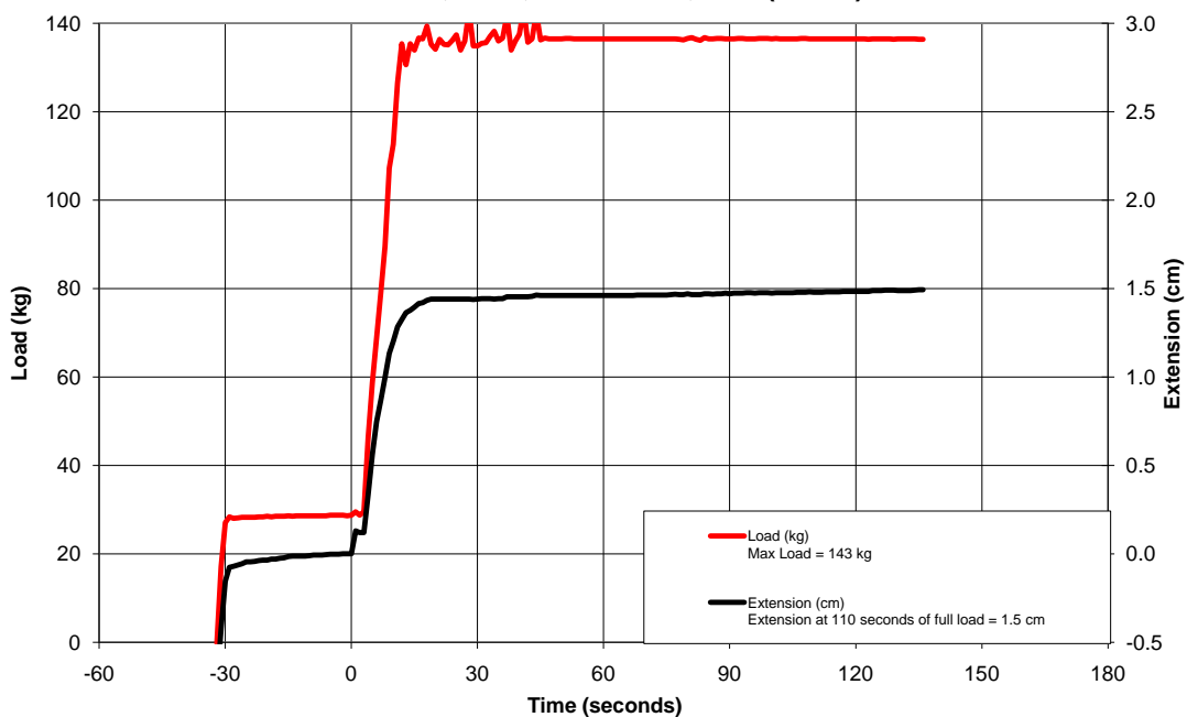
Low Temperature Retention Testing 03/11/11 JIAN171, MHR, LS2 MX453, XXL (64 cm)
