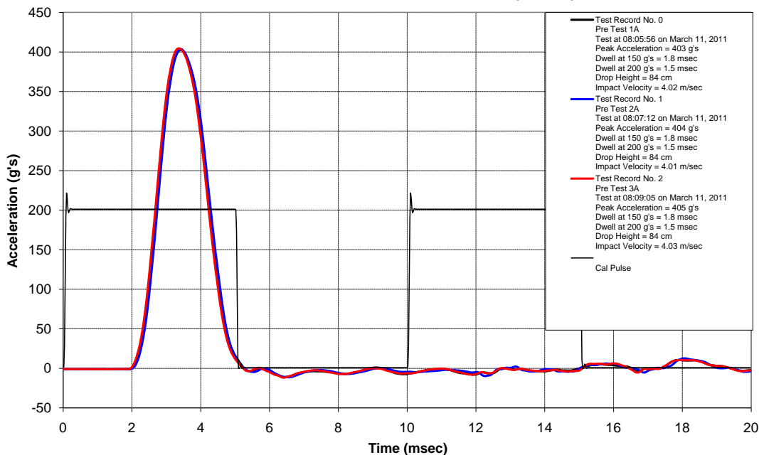
Impact Testing JIAN171, MHR LS2 MX453, XXL (64 cm)
