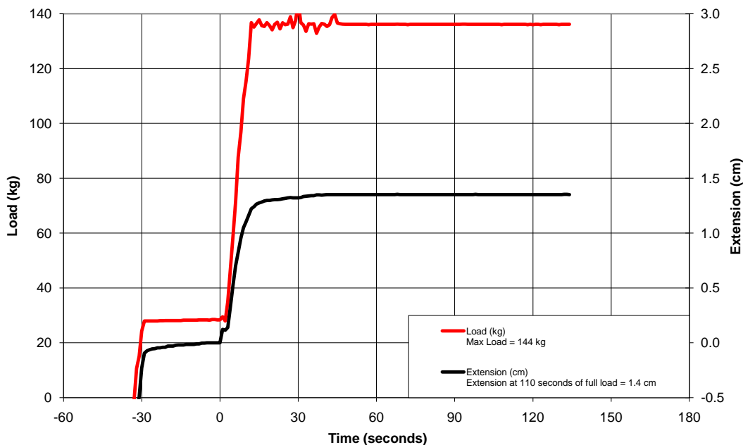
Ambient Temperature Retention Testing 03/11/11 JIAN171, MHR, LS2 MX453, XXL (64 cm)
