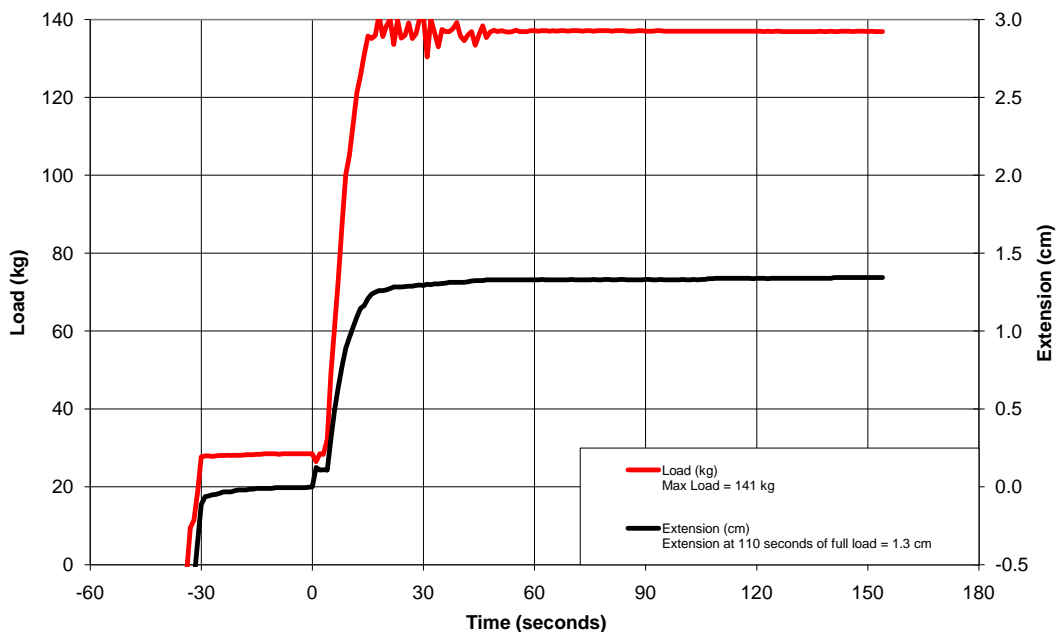
Ambient Temperature Retention Testing 02/11/11 JIAN165, MHR, LS2 FF453, M (58 cm)
