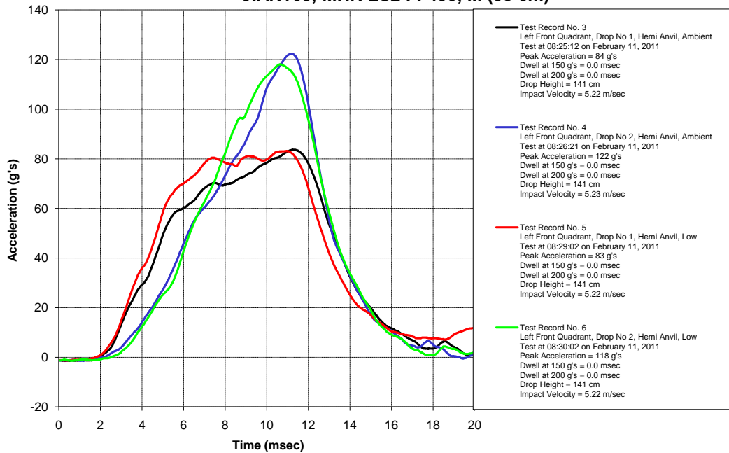
Impact Testing JIAN165, MHR LS2 FF453, M (58 cm)
