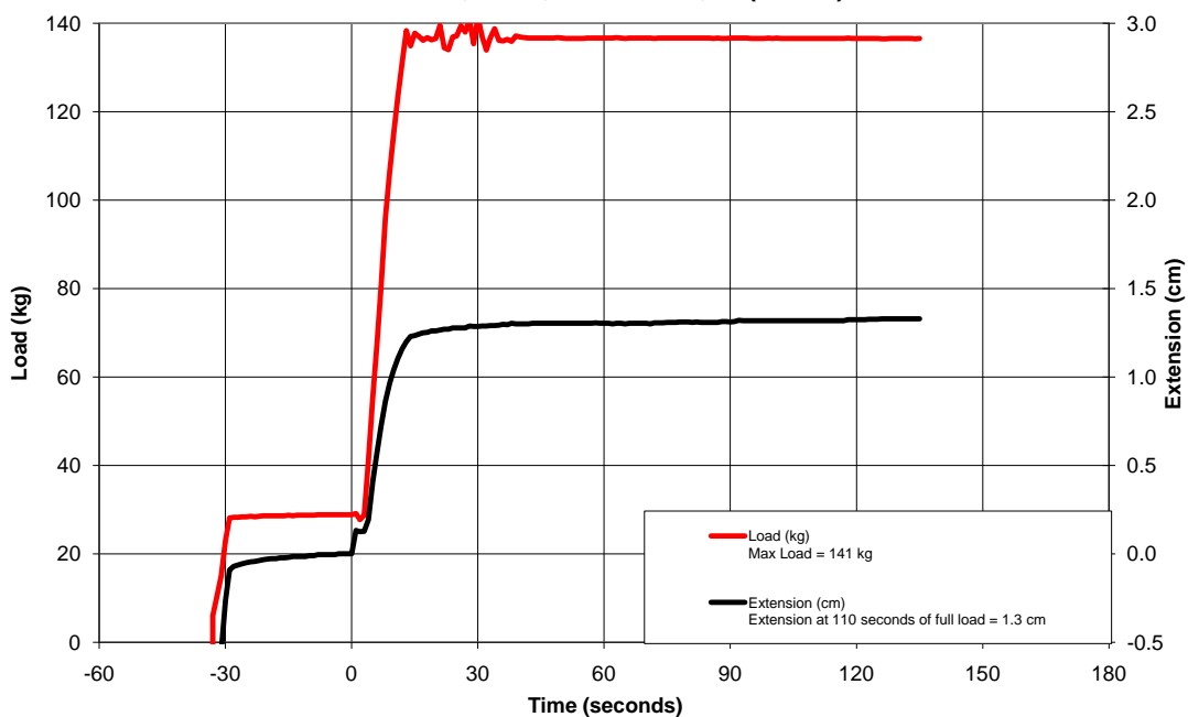
Low Temperature Retention Testing 02/11/11 JIAN165, MHR, LS2 FF453, M (58 cm)
