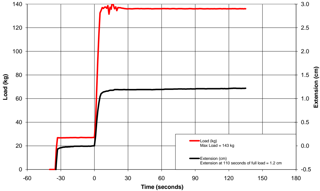
Ambient Temperature Retention Testing 02/18/10 JIAN124, MHR, MX442, XXL
