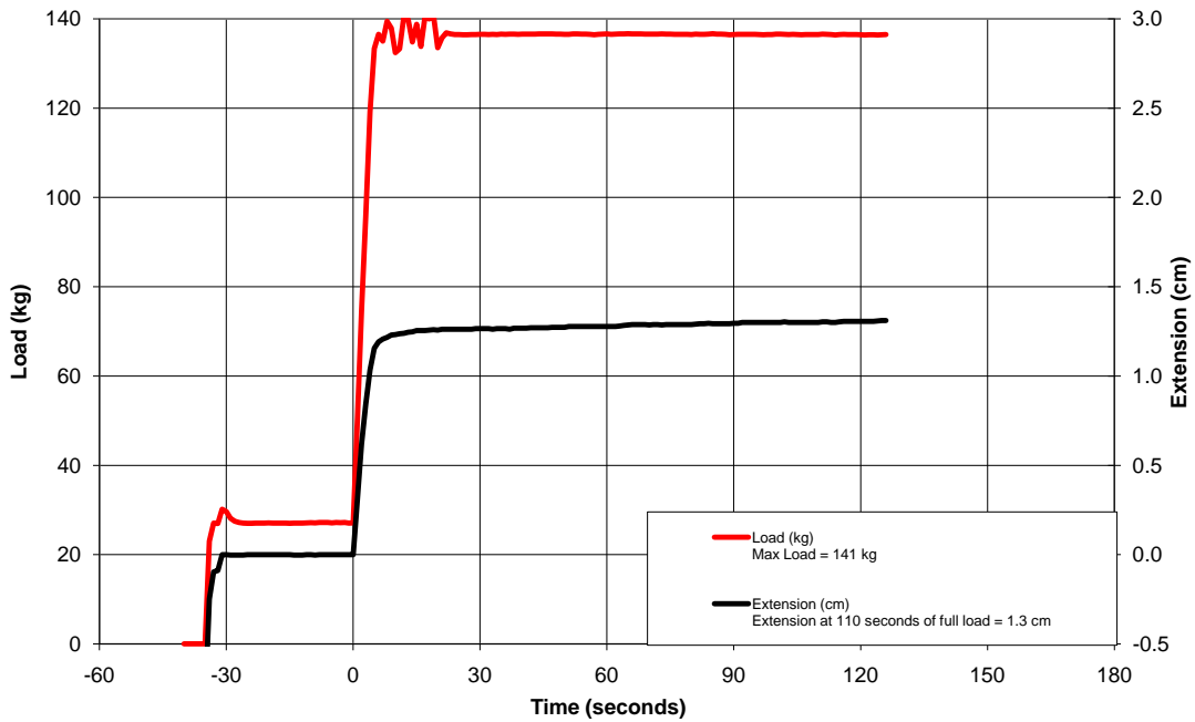
Low Temperature Retention Testing 02/18/10 JIAN124, MHR, MX442, XXL
