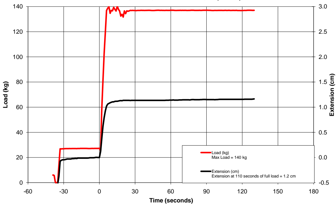
Low Temperature Retention Testing 02/24/10 JIAN126, MHR, Tuzo MX 422, S (56cm)
