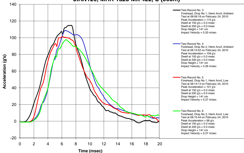
Impact Testing JIAN126, MHR Tuzo MX 422, S (56cm)
