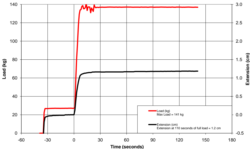
Ambient Temperature Retention Testing 02/24/10 JIAN126, MHR, Tuzo MX 422, S (56cm)
