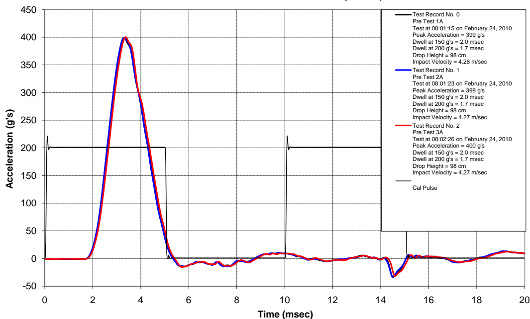
Impact Testing JIAN126, MHR Tuzo MX 422, S (56cm)
